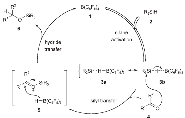
Scheme 1. The Piers mechanism of the B(C_6F_5)_3 -catalyzed hydrosilylation of carbonyl compounds.
