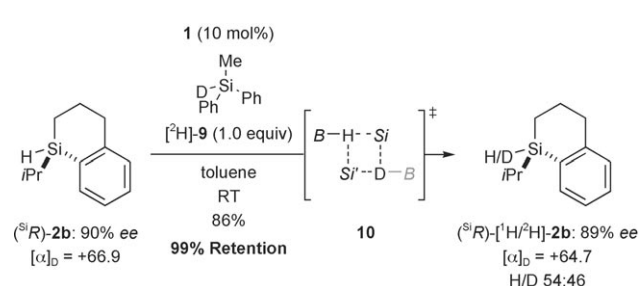
Scheme 4. Racemization-free scrambling in the absence of a Lewis base: No support for free silylium ions [ B = B(C_6F_5)_3 and Si or Si^* = R_3Si ].
