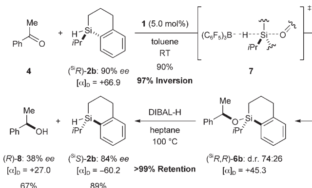
Scheme 3. Two-step stereochemical analysis: An inversion-retention pathway.
