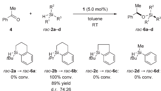
Scheme 2. Screening of suitable chiral probes.
